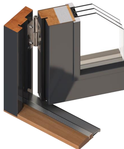
Threshold 35mm as option
